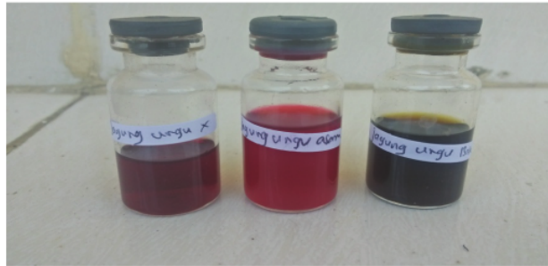
Figure 2. The result of anthocyanin color-test
